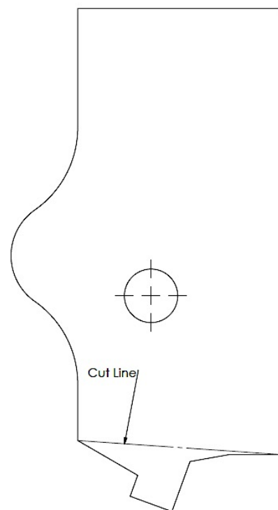
Figure 1- Left Frame Guard Profile. Depicts the bottom of the left frame guard plastic and the optimal cut line to allow the Fastway footpegs to function properly. NOTE: Not drawn to scale, to be used for reference.
